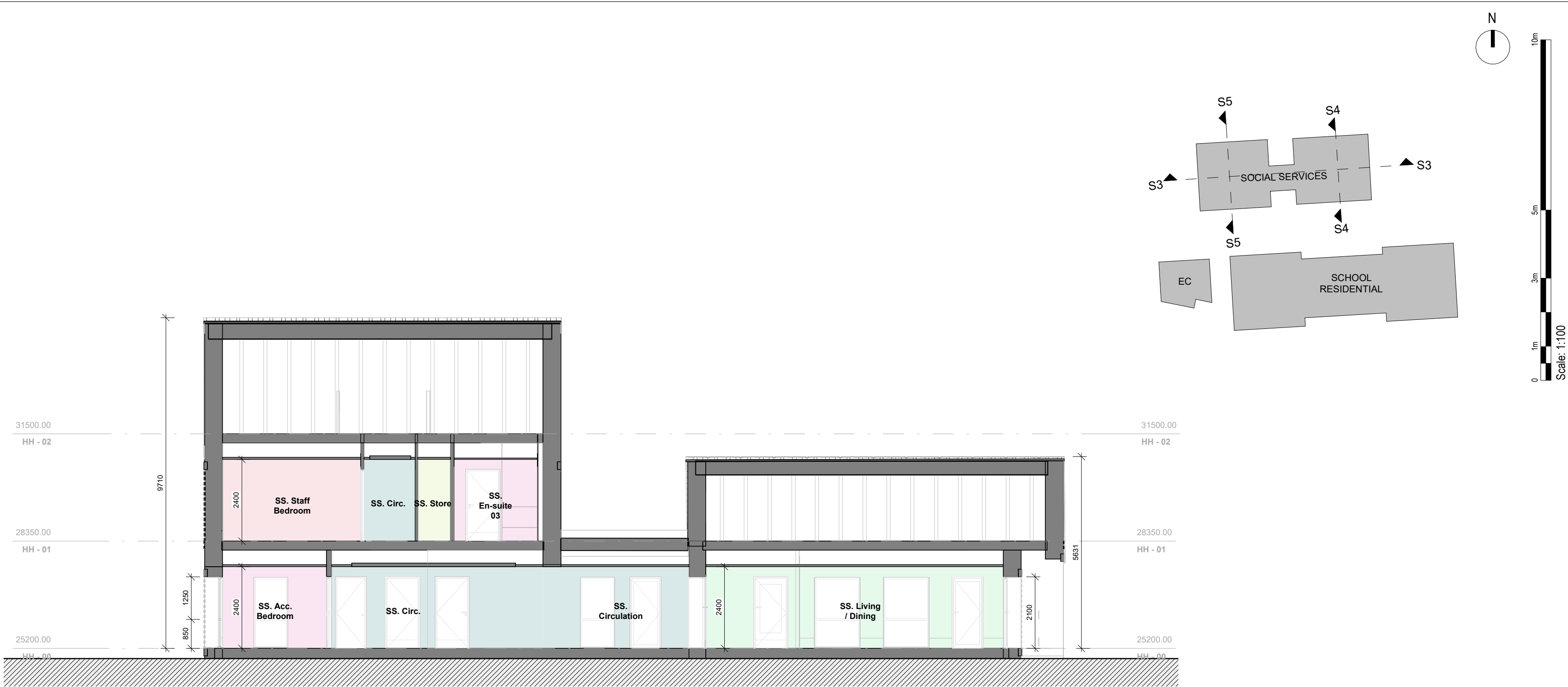
Section 3_Planning Scale: 1 : 100
