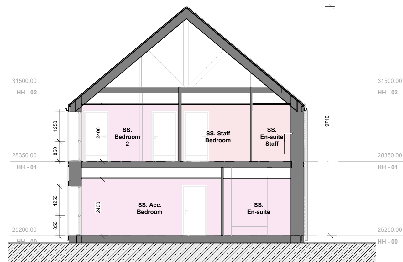
Section 5_Planning Scale: 1 : 100
