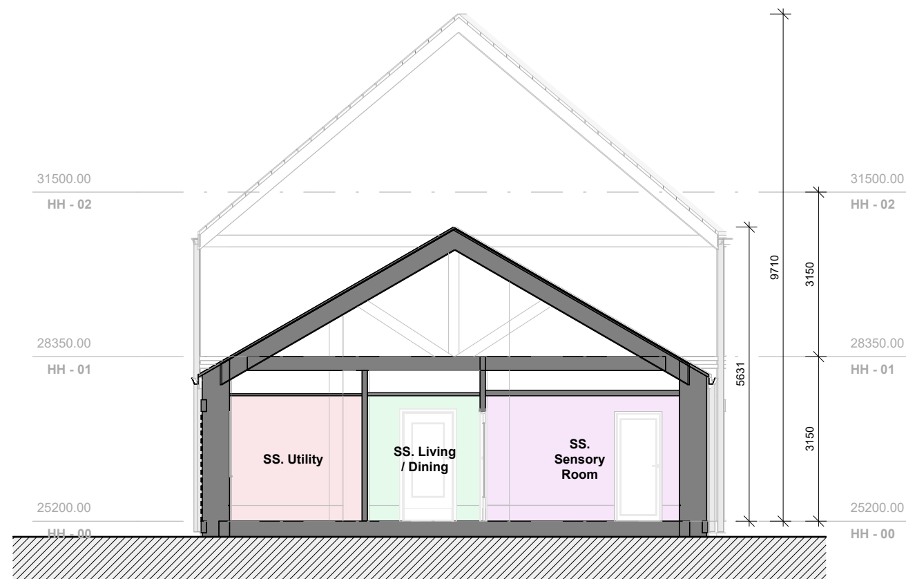
Section 4_Planning Scale: 1 : 100
